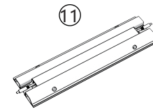
Power-side extension pole assembly x 1
